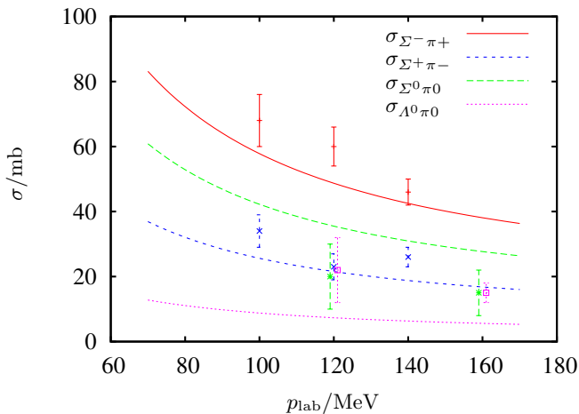
Fig. 1. Cross-sections for the inelastic reactions K^-p \rightarrow Y\pi , where Y\pi = \Sigma^-\pi^+, \Sigma^+\pi^-, \Sigma^0\pi^0 and \Lambda^0\pi^0 .
